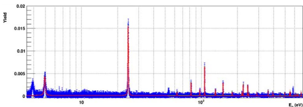
Fig. 2. Experimental capture yield of the ^{171}\text{Tm}(n,\gamma) measurement at CERN n_TOF.
