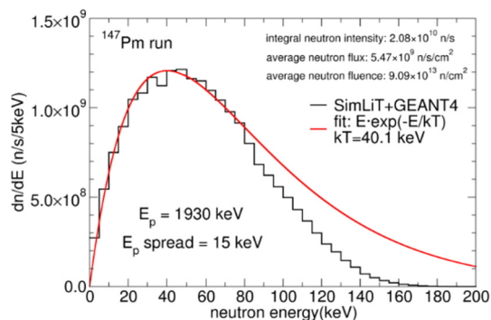
Fig. 2. Simulated neutron spectrum impinging on the ^{147}\text{Pm} target according to the SimLiT-Geant4 simulations, including a fit to a Maxwell-Boltzmann distribution at 40.1 keV.
