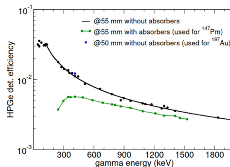
Fig. 4. Efficiency curves of the HPGe detector at 55 mm distance used for the ^{147}\text{Pm} target (with and without absorbers) and at 50 mm distance used for ^{197}\text{Au} .
