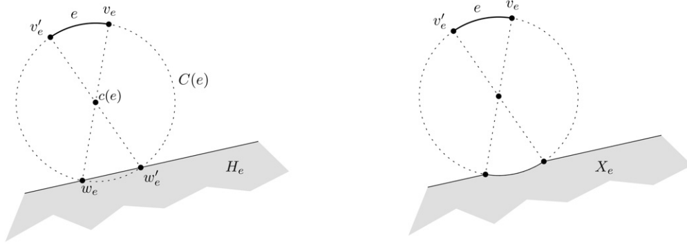
Fig. 3. Left: notation concerning an edge e . Right: the region X_e .
